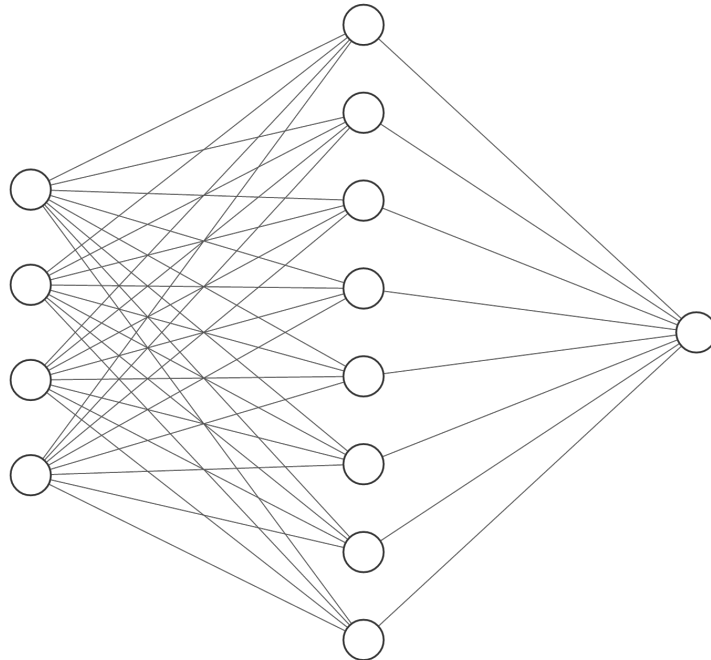
Figure 10: Structural diagram of the feed-forward MLP engine, illustrating the 4 \rightarrow 8 \rightarrow 1 fully connected neural network layers utilized by the local client inference system.
